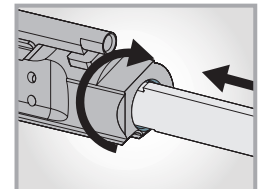
4 & 5: Two interior bolt carrier surfaces
