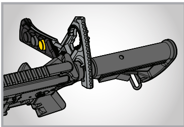
Castle nut wrench specifically designed to work around MIL-SPEC and aftermarket end plates
