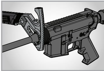
Barrel nut wrench precisely fits all standard MIL-SPEC barrel nuts
