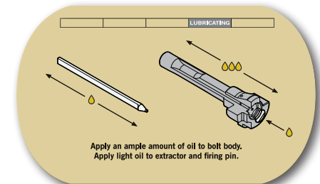
Critical lubrication points are highlighted and explained
