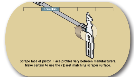
Where to scrape carbon from critical bolt carrier assembly surfaces
