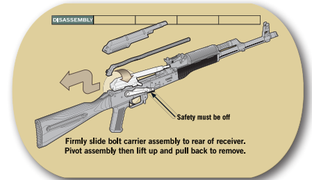
Step-by-step field stripping instructions
