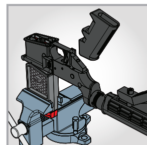
Invert lower receiver for changing pistol grips
